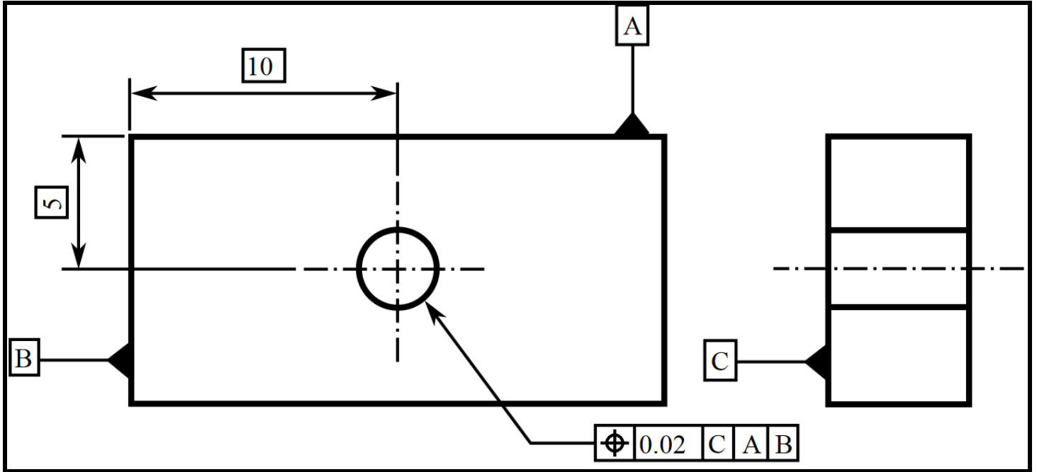
Figure 1 – Geometric Dimensioning and Tolerancing example
